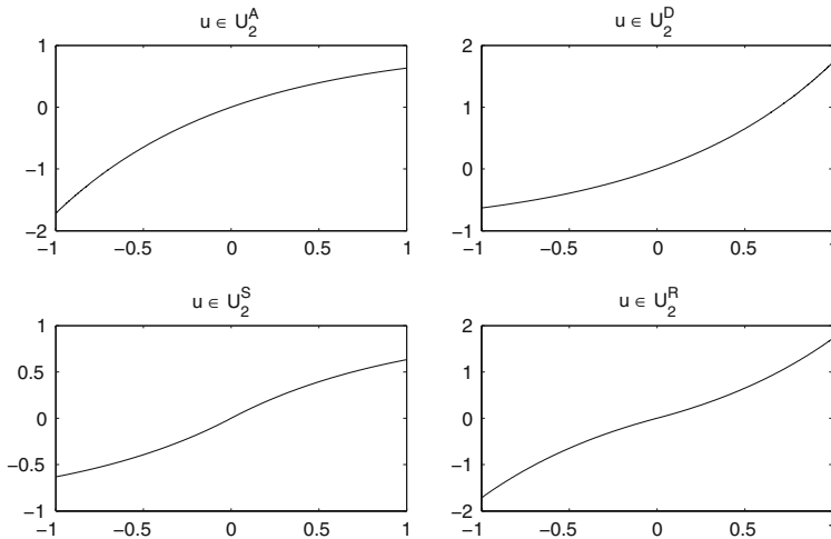
Fig. 1 Functions in U_2^A , U_2^D , U_2^S and U_2^R
