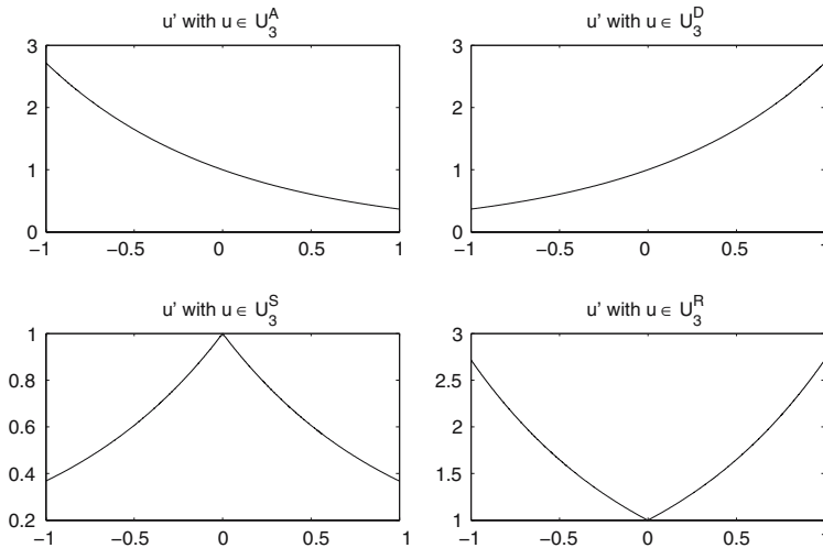
Fig. 2 Derivatives of Functions in U_3^A , U_3^D , U_3^S and U_3^R
